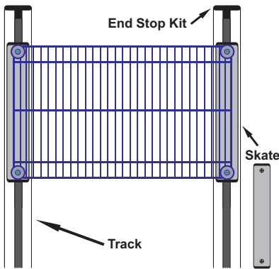
SINGLE UNIT TRACK SYSTEM (Top View)
