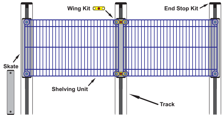
DOUBLE UNIT TRACK SYSTEM (Top View)
